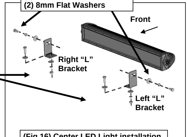
(Fig 16) Center LED Light installation
