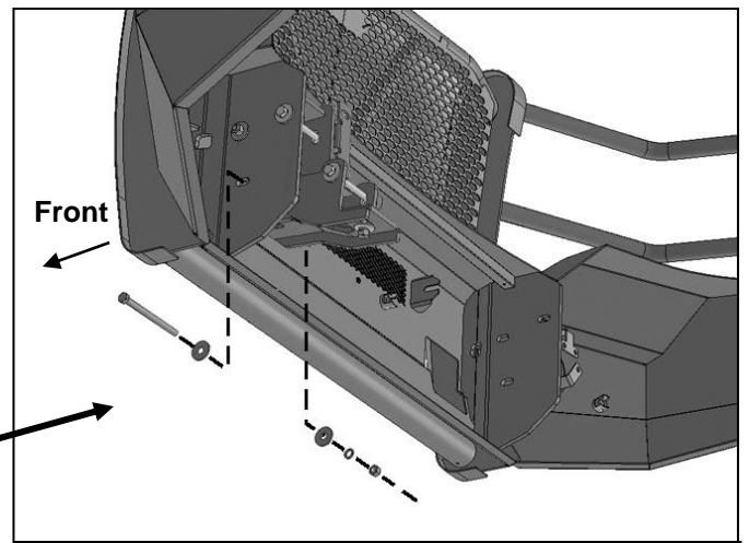
(Fig 13) Insert long 12mm x 160mm Hex Bolt with Flat Washer through Bumper, Bracket and tow hook. Back of driver side of Bumper illustrated
