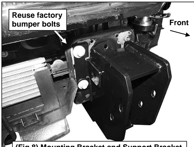
(Fig 8) Mounting Bracket and Support Bracket
