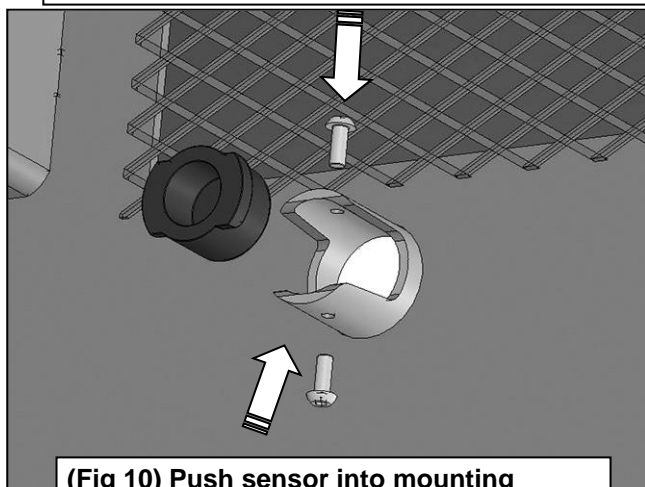
(Fig 10) Push sensor into mounting sleeve. Use 4mm Screws to lock sensor
