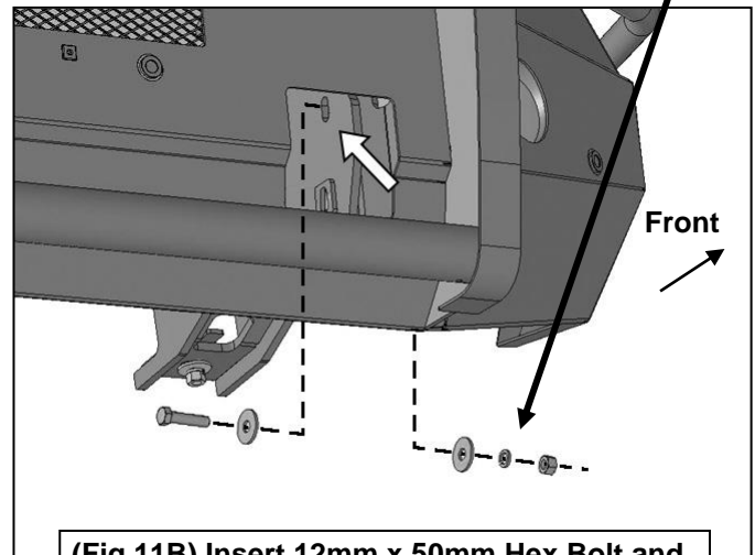
(Fig 11B) Insert 12mm x 50mm Hex Bolt and Flat Washer into opening for tow hook and out through inside slot in top of Bracket. Front of driver side of Bumper illustrated
