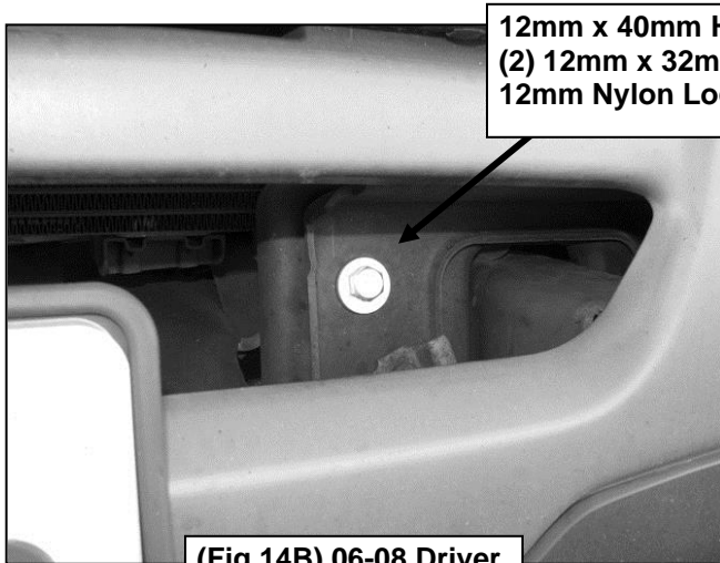
(Fig 14B) 06-08 Driver side bumper bracket
