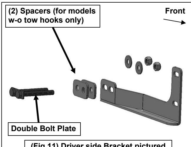
(Fig 11) Driver side Bracket pictured
