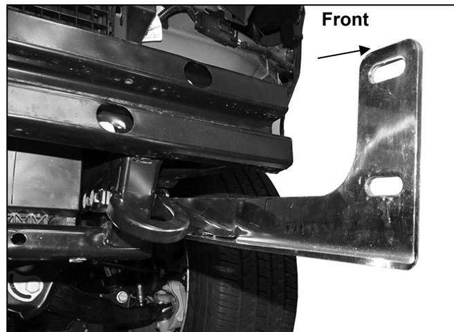
(Fig 12) Driver side Bracket installed over tow hook, Spacers are not required. Installation pictured without bumper for instruction purposes only
