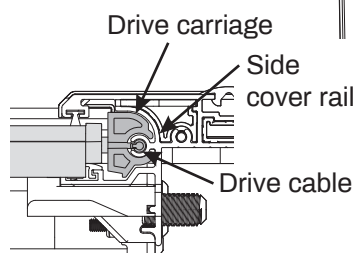
Rear section view
