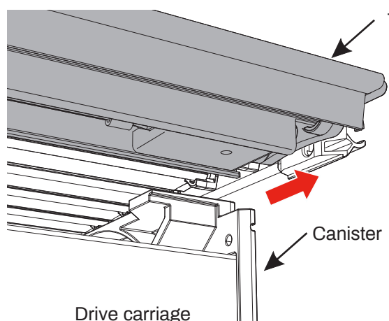
Tail Panel
