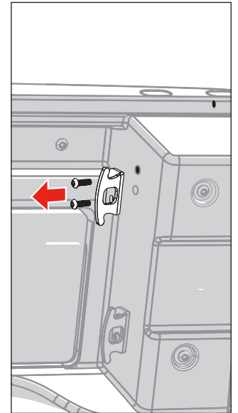
Upper Tie-Downs Near Tailgate
