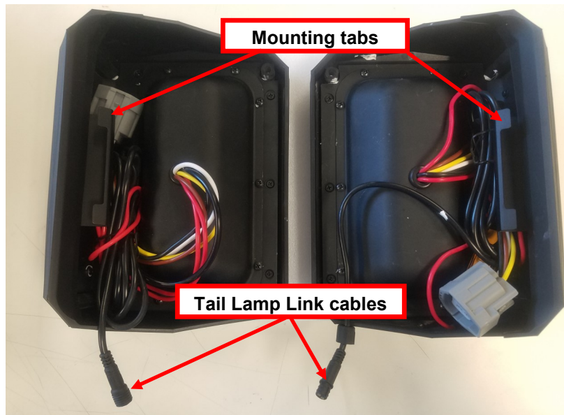
Figure 3: Mounting tab and linking cable.
