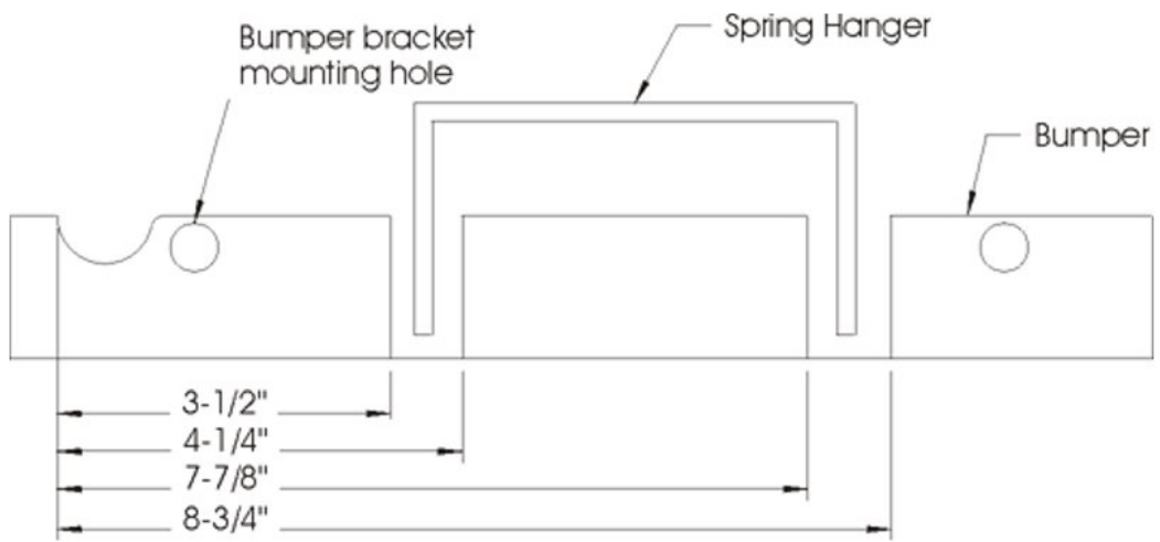
Bumper cutouts
