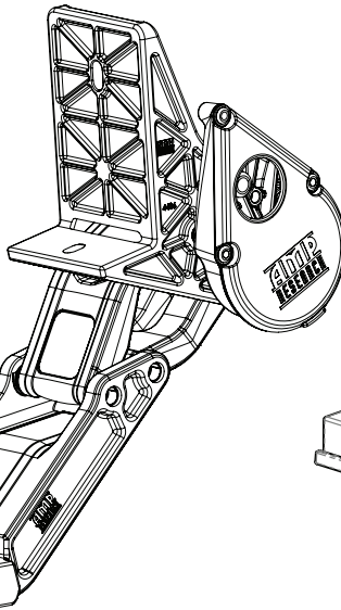
3 Passenger Side Motor Linkage Assembly
