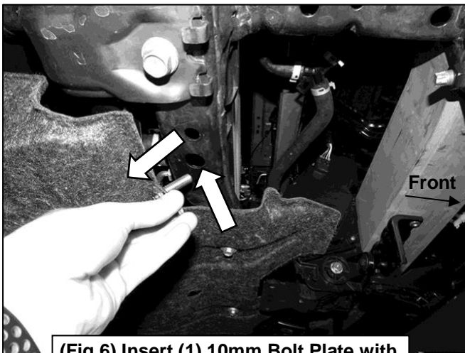
(Fig 6) Insert (1) 10mm Bolt Plate with Fish Wire into the large hole the crossmember and out the smaller hole towards the side of the vehicle
