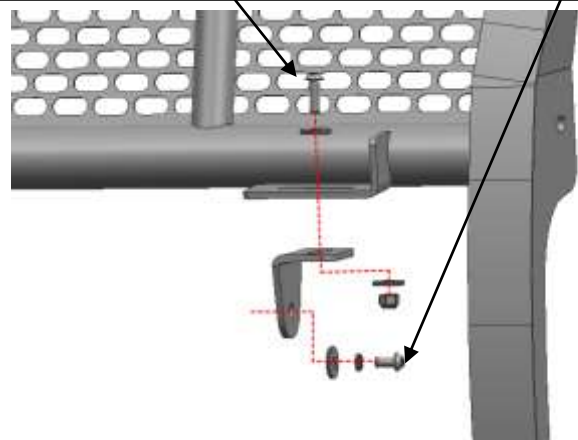
(Fig 20) Attach LED Lamp Bracket to Grille Guard Main Body
