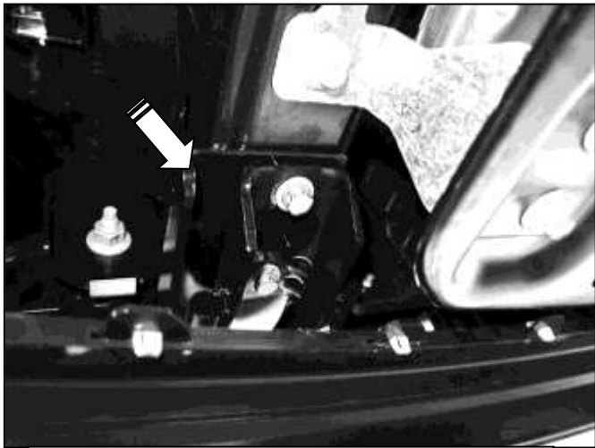
(Fig 7) Attach the driver/left Frame Mounting Bracket to the bottom of the frame. Reinstall tow hook (if equipped) over the Bracket
