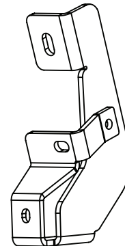
26 x2 Rail Mounting Bracket
