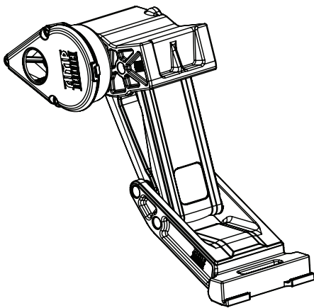
Motor Linkage assembly
