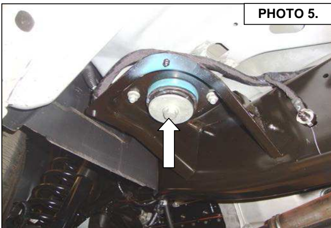
Remove this bolt and washer to attach the front auxiliary bracket. Front driver's side.
