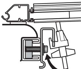
Cab Clamp
