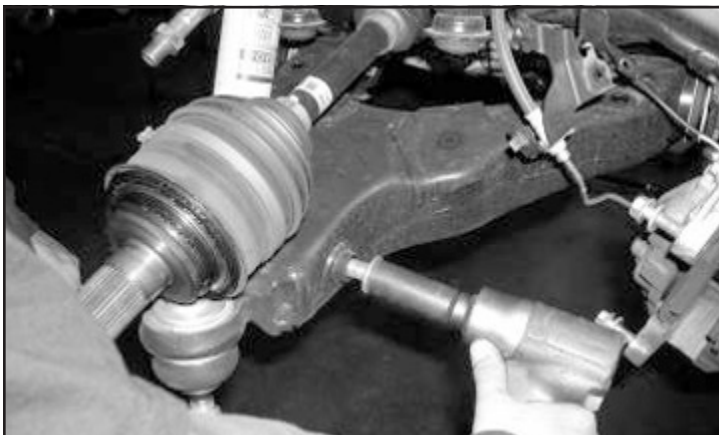
FIGURE 28 - STEP 10
