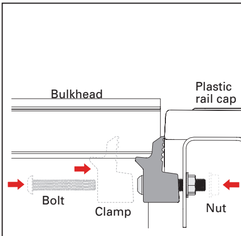
Installing Clamp
