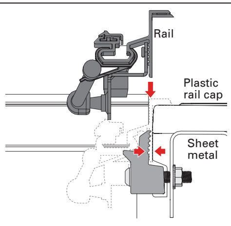
Installing Rail
