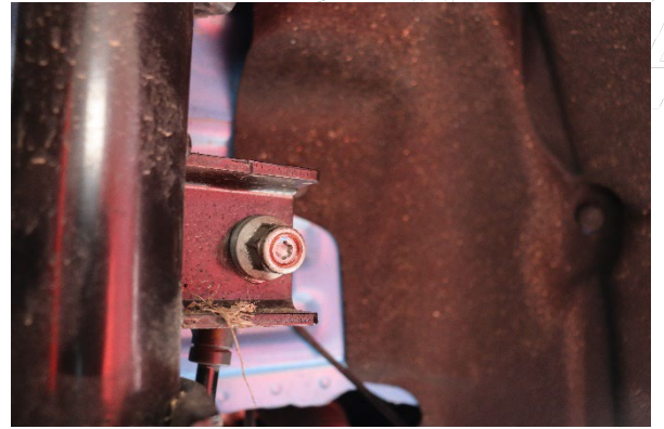
14. Reinstall the end link nut with a 18mm socket.
