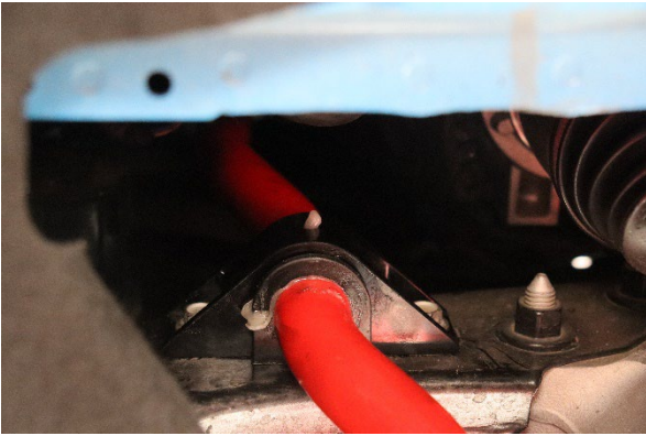
13. With the bar in the proper position install the provided brackets and secure them with the OE hardware using a 15mm socket.
