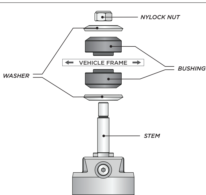
MEDIUM DUTY STEM BUSHING DIAGRAM
