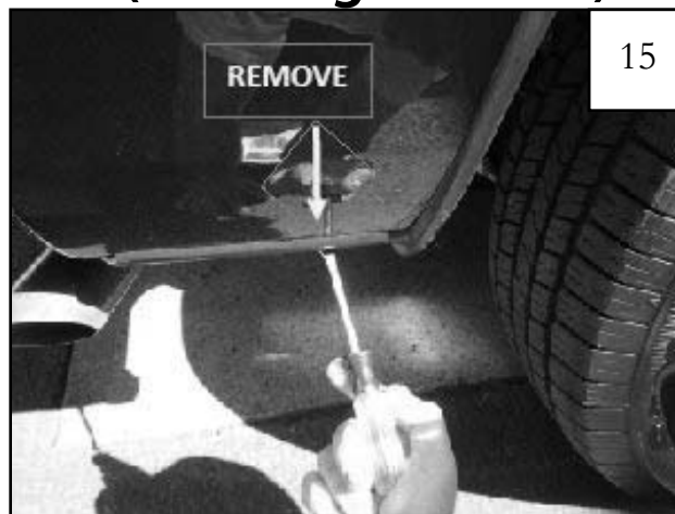
2012 - 2014 Models Only (Optional): Remove inner piece at bottom rear of wheel well using a pry tool.
