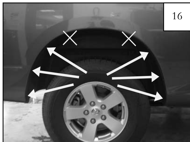
Remove these six factory installed screws using an 8mm socket wrench. Keep screws for installation of the rear flare. X's indicate a factory screw that will not be removed.
