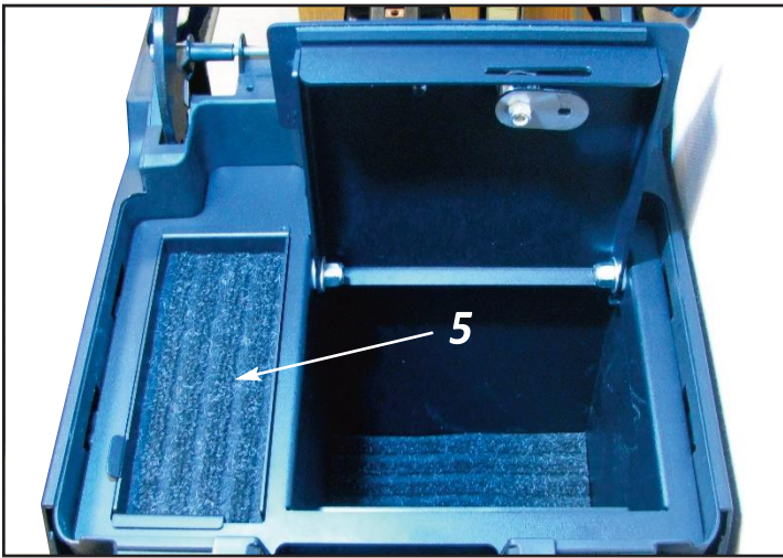
5. Align the supplied console safe tray and carpet insert into the upper opening in the console safe (prototype insert shown, production insert may differ).
