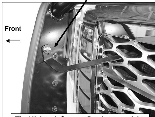
(Fig 16) Attach Support Bracket to upright
