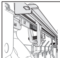
Rear clamp installed with step spacer
