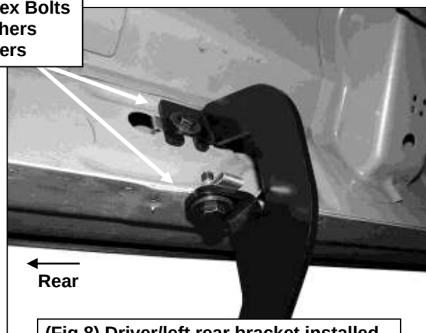
(Fig 8) Driver/left rear bracket installed
