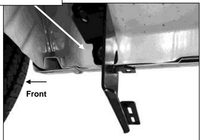
(Fig 16) Passenger/right side front Bracket
