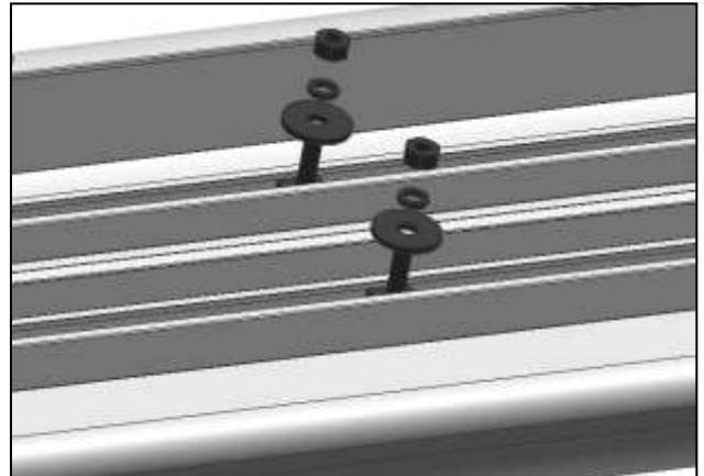
(Fig 9) Insert T-Bolt Plates into channels
