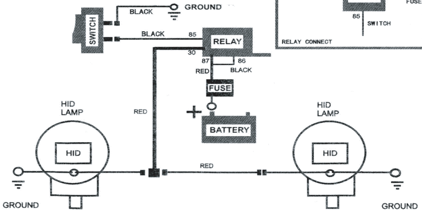
WIRE HARNESS DIAGRAM FOR 2 LIGHTS
