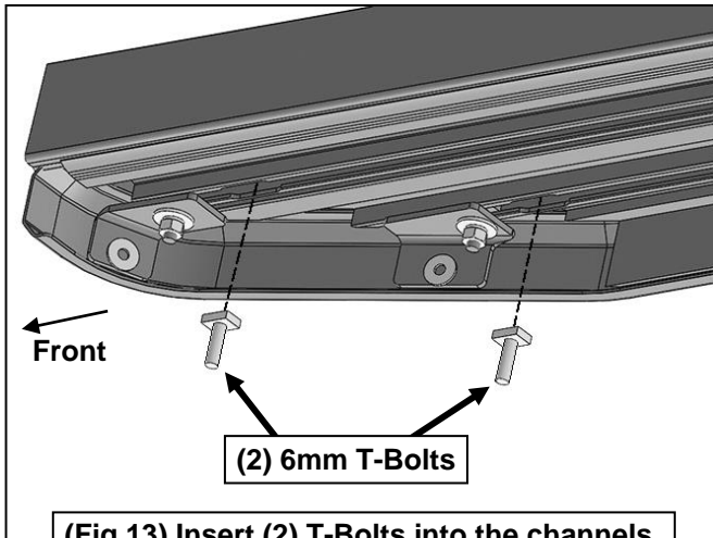
(Fig 13) Insert (2) T-Bolts into the channels on the bottom of the Running Board
