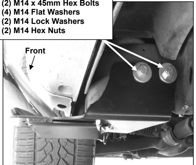
(Fig 3) Driver side front Mounting Bracket pictured after plastic cover removed
