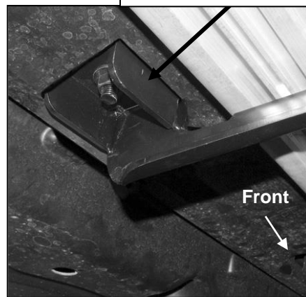
(Fig 10) Passenger side center Bracket installed
