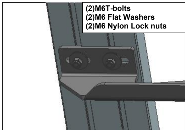
(Fig 3) Bracket Installation
