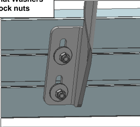
(Fig 13) Bracket installation
