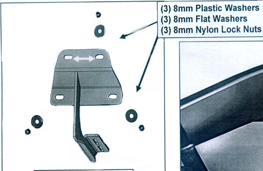
(Fig 5) Typical Bracket installation illustrated
