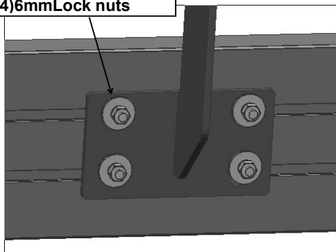
(Fig 6) Bracket installed
