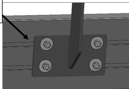
(Fig 4) Driver/left front mounting Bracket
