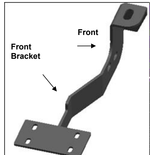
(Fig 2) Passenger side front Brackets
