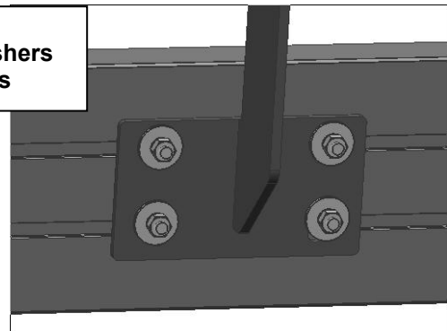
(Fig 11) Passenger side Bracket Installation
