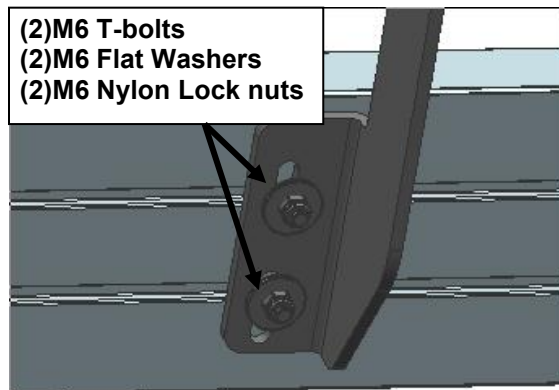
(Fig 6) Bracket Installation (example only)
