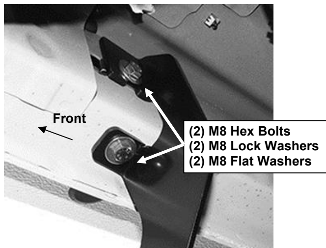
(Fig 4) Passenger side front Bracket installation(example only)
