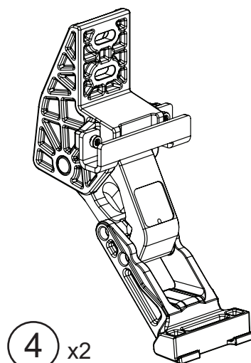
Front Idler Linkage Assembly
