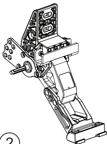
Rear Motor Linkage Assembly (Driver)
