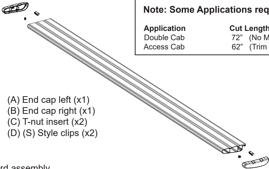
Running Board assembly
