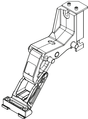
Idler Linkage Assembly
