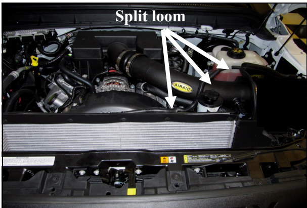
10. Slide the 20” section of Split Loom (#8) over the Coolant line to protect it from chaffing on the intake tube.
