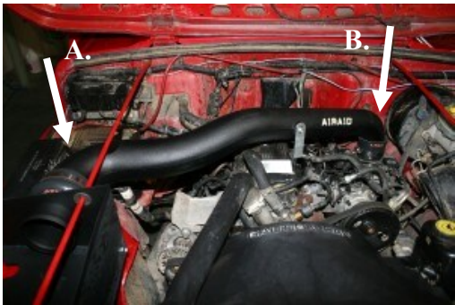
19. A.) Install the large end of the Airaid Intake Tube into the hump hose. B.) Now slide the small end into the reducer on the throttle body.
