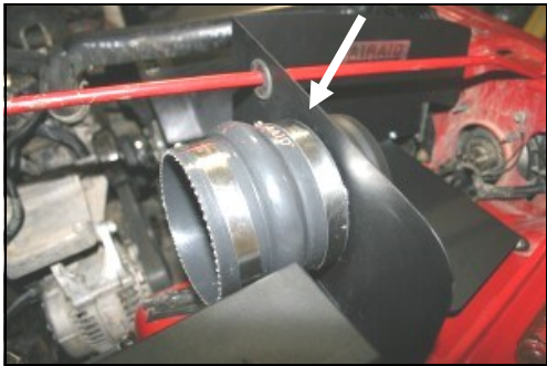
16. Install the hump hose (#5) onto the back side of the CAD tube using two #72 hose clamps (#17). Tighten only the hose clamp on the metal tube for now.
