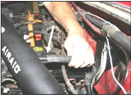
21. Re-connect the breather hose to the Airaid Intake Tube.
