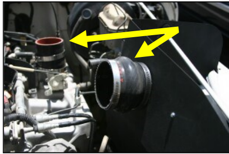
15. Install hump hose on CAD with #52 hose clamps, and the coupler on the throttle body with #44 hose clamps as shown.
