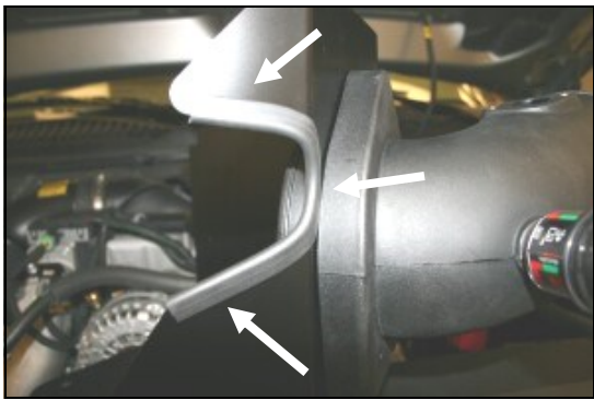
10. Install the provided rubber trim (#13) on the CAD as shown.
