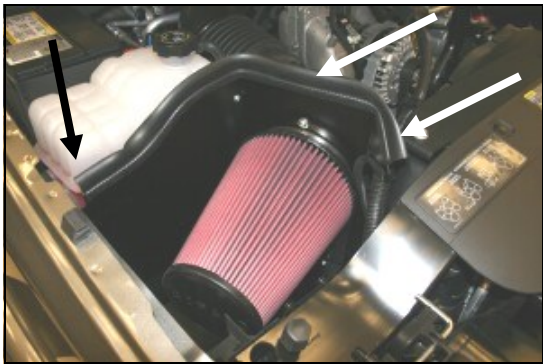
13. Install the Airaid Premium Filter (#1) onto the Airaid intake tube (#4), and tighten the hose clamp. Now install the provided weather strip (#5) on the top of the CAD. For ease of installation, start near the fender and work your way towards the radiator.
