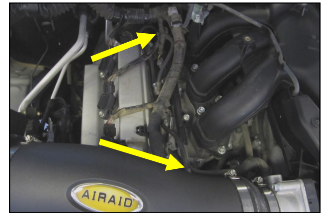
40. replace the OEM vacuum line on the fuel pressure regulator with the supplied 20 1/2" 1/8" line (#12). Connect the 1/8" line to the small Fitting on the Intake tube.
