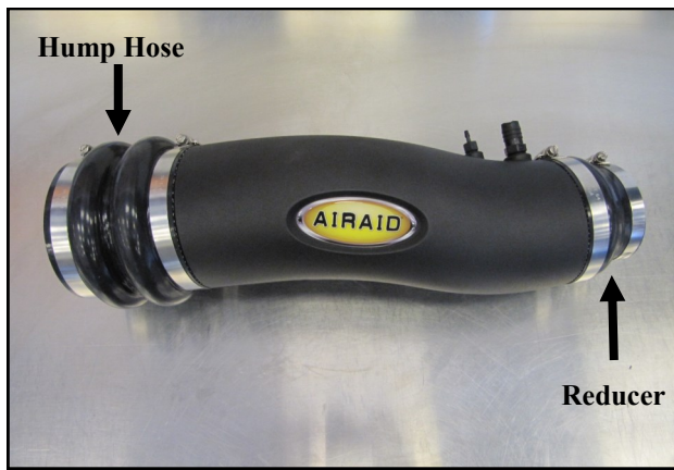
10. Slide the Hump Hose, and two #68 Hose Clamps onto the Intake Tube as shown. Slide the Reducing Coupler and the #48 and #64 Clamps on the other end of the Intake Tube. Leave the Clamps loose for now.
