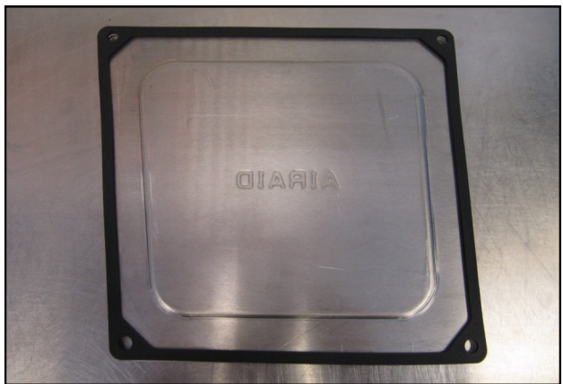
15. Place the Gasket onto the underside of the Air Box Lid and peel off the protective film. Mount the lid on the Air Box using four 1/4-20 x 1/2" Button Head Bolts, and 1/4" Flat washers.
