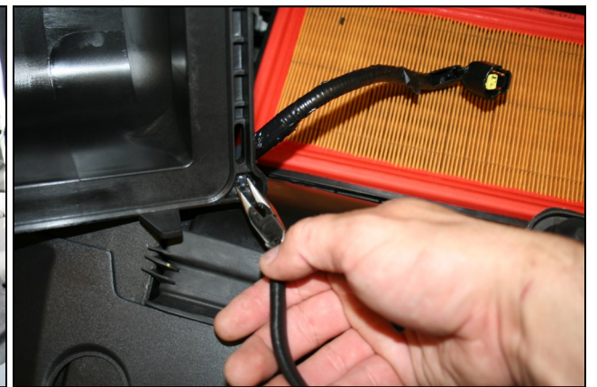
3. Using a pair of needle nose pliers, carefully compress the fins of the wiring harness anchor and pull it out of the air box lid.
