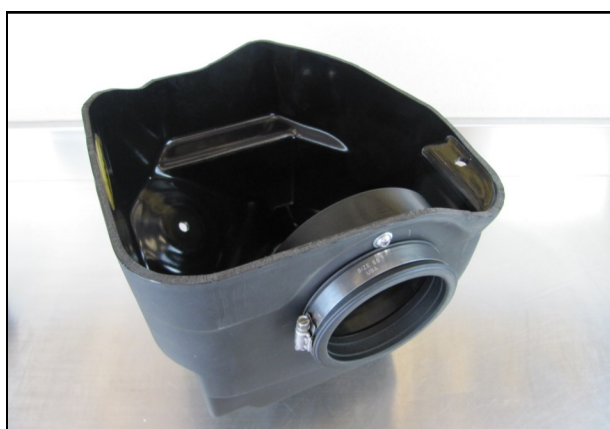
5. Slide the Coupler and Clamp onto the Filter Adapter as shown. Do not tighten the Clamp at this time.
