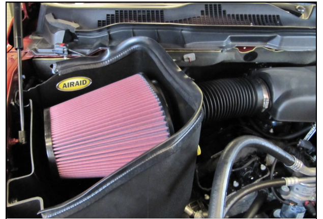
12. Install the Airaid Premium Filter onto the Filter Adapter inside the Cool Air Box. Install the Weatherstrip onto the Cool Air Box as shown, with the contour rolling away from the Filter. Apply the Airaid Bubble Decal inside the Airbox as shown.
