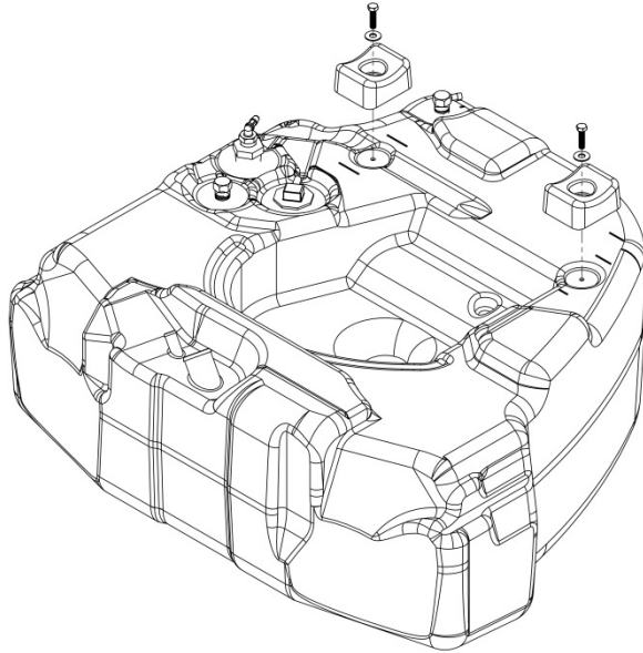
(Fig. 9) Exploded view showing spacers (01 0000 0130) required on 11+ GM attaches vehicles.
