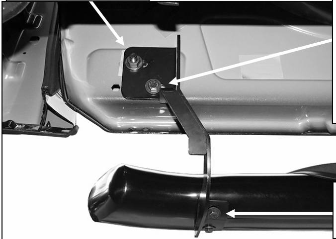
(Fig 13) Driver/Left rear Mounting Bracket
