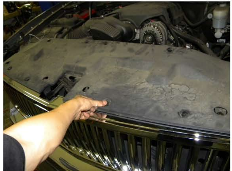
10. Replace plastic radiator cover and (8) plastic clips
